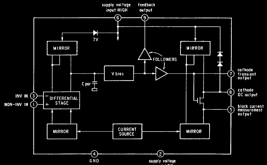
CR BOARD IC701 TDA6101Q
